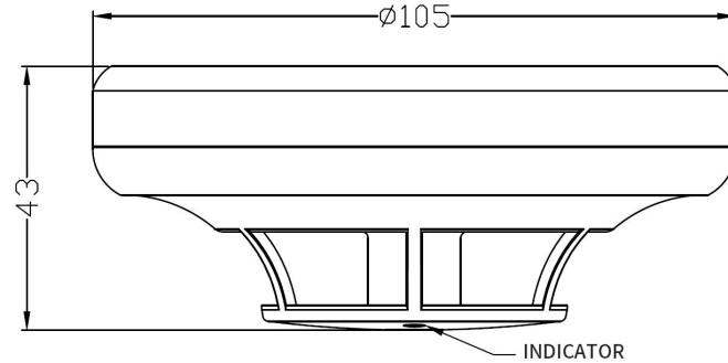
Figure.1 (Unit: mm)
